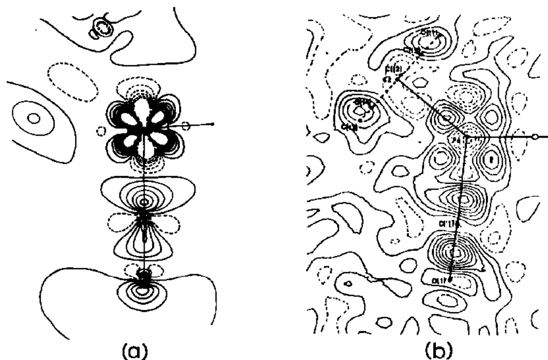
Fig. 3. Deformation density distribution in \text{trans}[\pi\text{-C}_5\text{H}_5)\text{Fe}(\text{CO})_2]_2 from ref. 12. Section containing Fe-Fe line and the terminal carbonyls. (a) Theoretical, contour interval 0.2 \text{ e}\text{\AA}^{-3} . Dashed contours negative. (b) Experimental, contour interval 0.1 \text{ e}\text{\AA}^{-3} . Broken contours negative.
