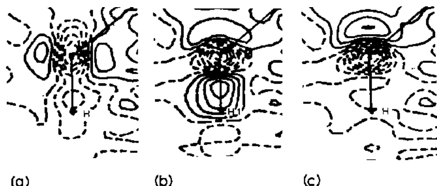
Fig. 2. Deformation maps of CH ligand in \text{Co}_3\text{CH}(\text{CO})_9 . Contours as in Fig. 1. (a) Fragment deformation map subtracting 2\text{II} density. (b) Atom deformation map. (c) Fragment deformation map subtracting 4\Sigma density. From ref. 8.
